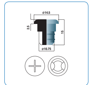
C1546 - Crenelated stopper
